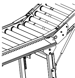
KE500 – Grind, driven
