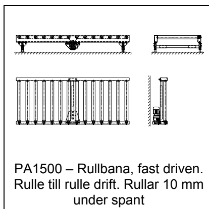
PA1500 – Rullbana, fast driven/driven ackumulerande Typ FD/DA. Kedjedriven *
